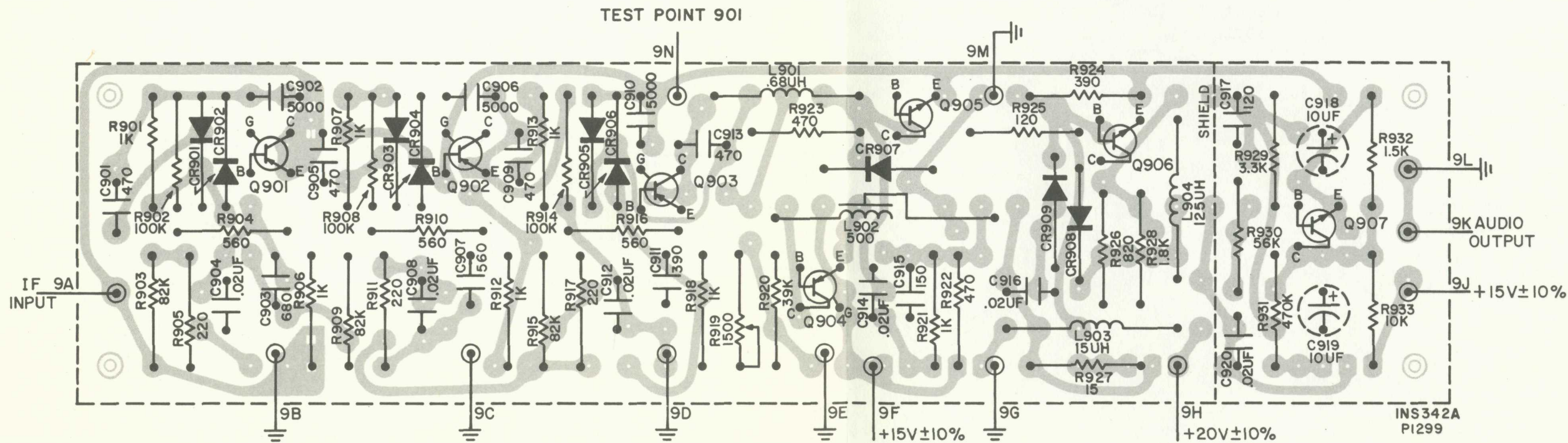
BOARD VIEWED FROM THE COMPONENT SIDE
